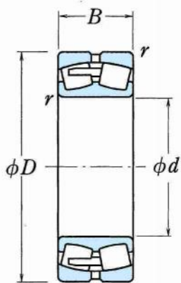
圓柱孔
