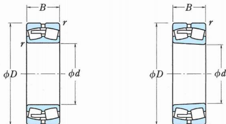
圓柱孔
