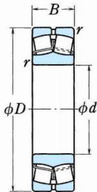
圓柱孔
